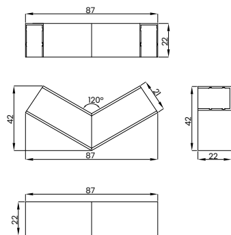
Conector "V"
